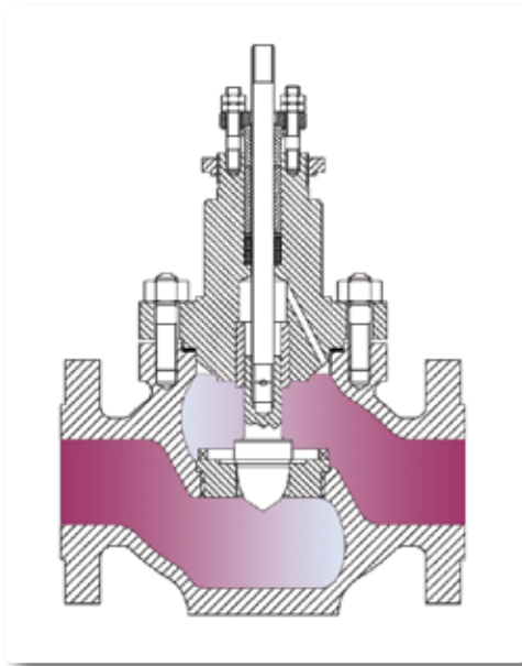
Contoured trim Metal to Metal
