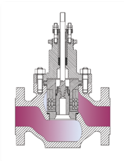
LR 3 Triple Stage Low Pressure Recovery
