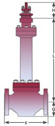
Valve with Bellows seal bonnet
