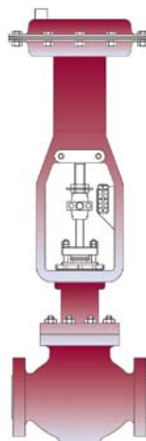
Series 110: Control valve with standard bonnet and direct acting actuator
