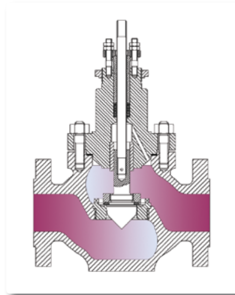
Contoured trim Soft Seated
