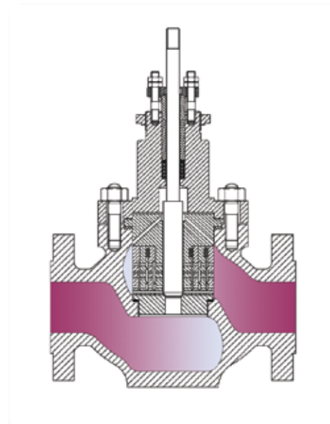
LR 4 Four Stage Low Recovery
