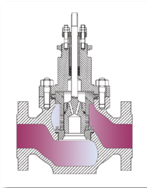
LR 1 Single Stage Low Pressure Recovery
