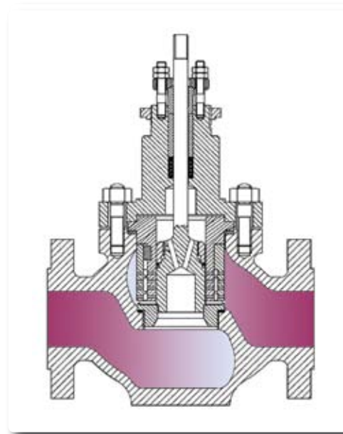
LR 2 Double Stage Low Pressure Recovery
