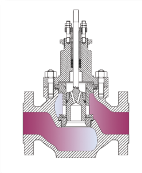
Ported trim Metal to Metal or Soft Seated
